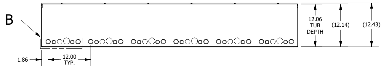
BOTTOM VIEW
