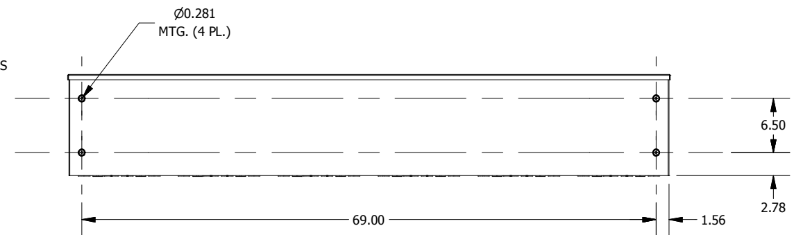
BACK VIEW
