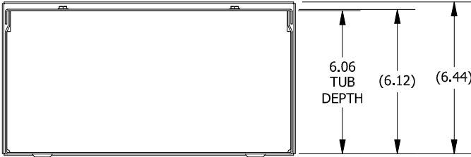
BOTTOM VIEW
