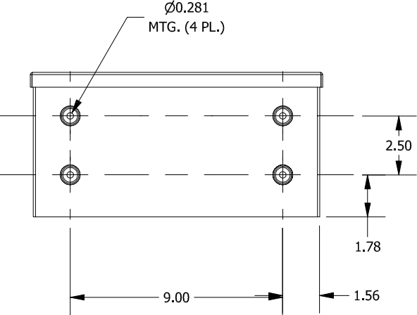
BACK VIEW
