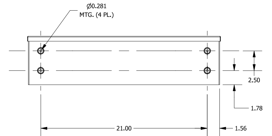
BACK VIEW
