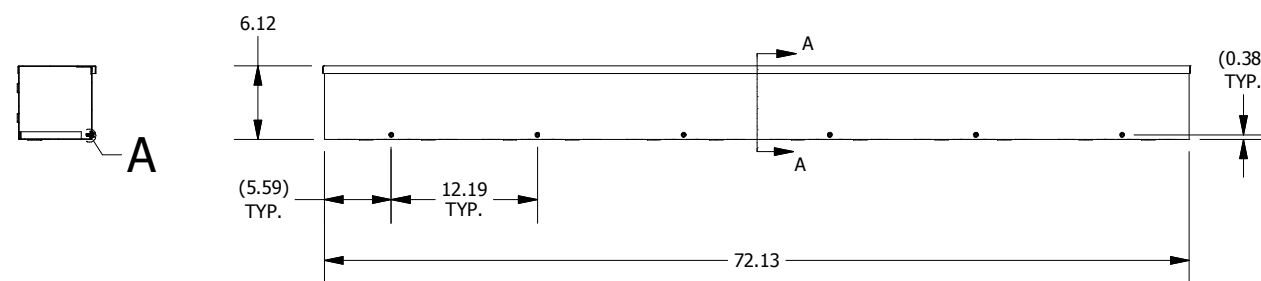
SECTION A-A (INSIDE RIGHT OF ENCL.)
