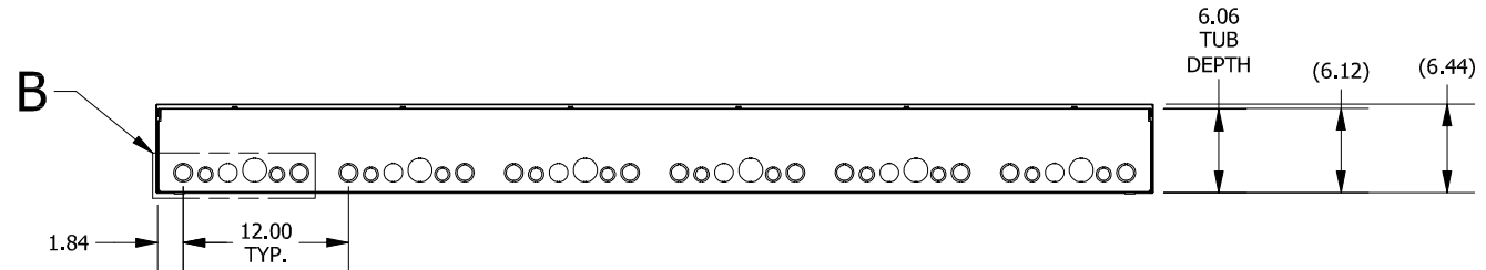
BOTTOM VIEW
