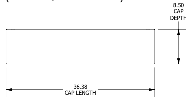
DETAIL A (3 PL.) (LID ATTACHMENT DETAIL)
