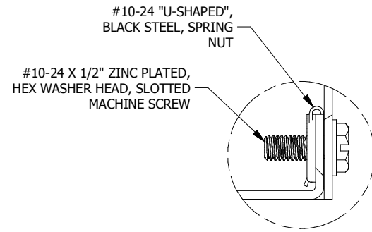
DETAIL A (3 PL.) (LID ATTACHMENT DETAIL)
