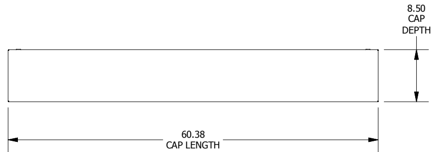
DETAIL A (5 PL.) (LID ATTACHMENT DETAIL)
