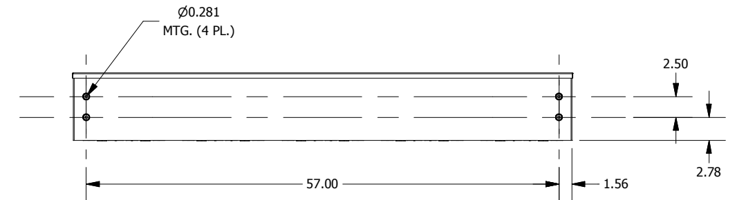
BACK VIEW
