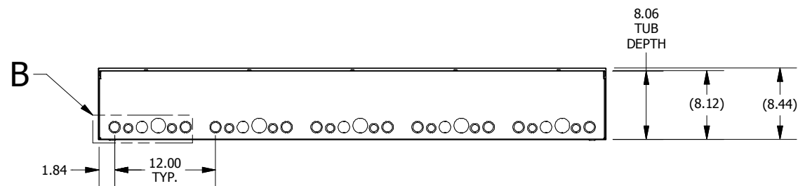
BOTTOM VIEW
