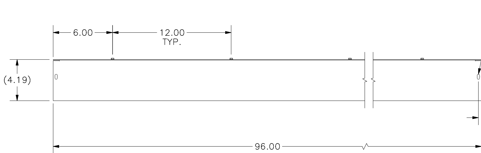
FRONT VIEW
