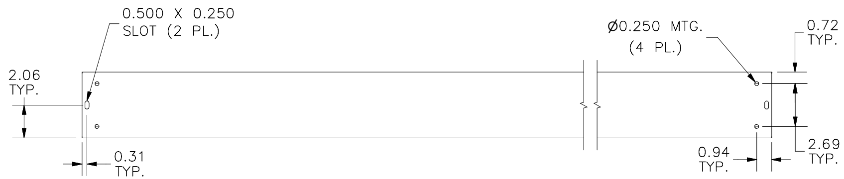
BOTTOM VIEW
