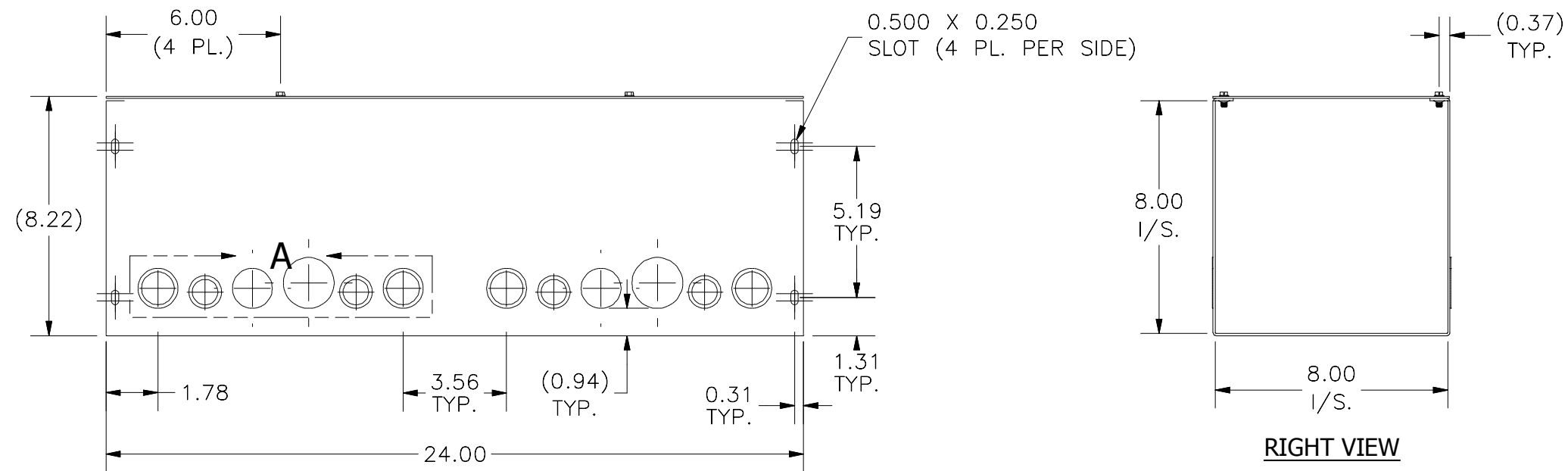
FRONT VIEW
