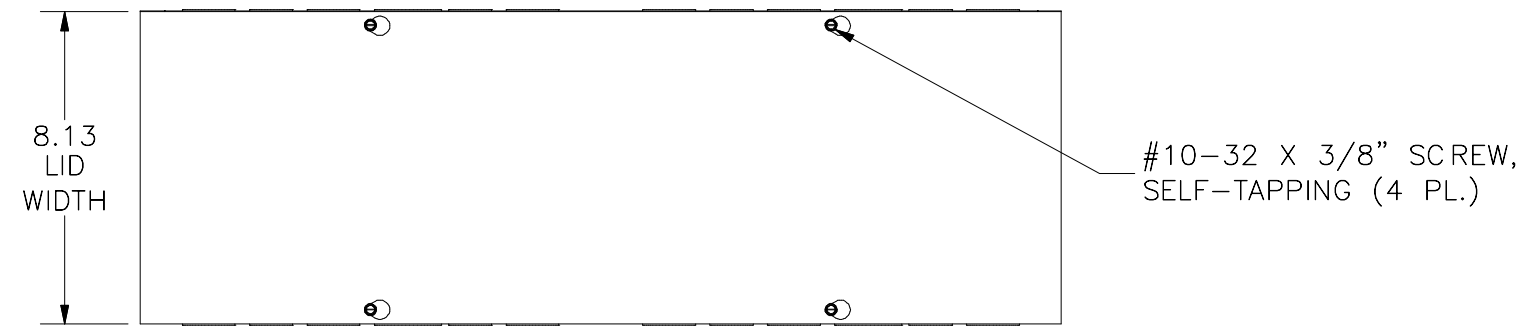
TOP VIEW
