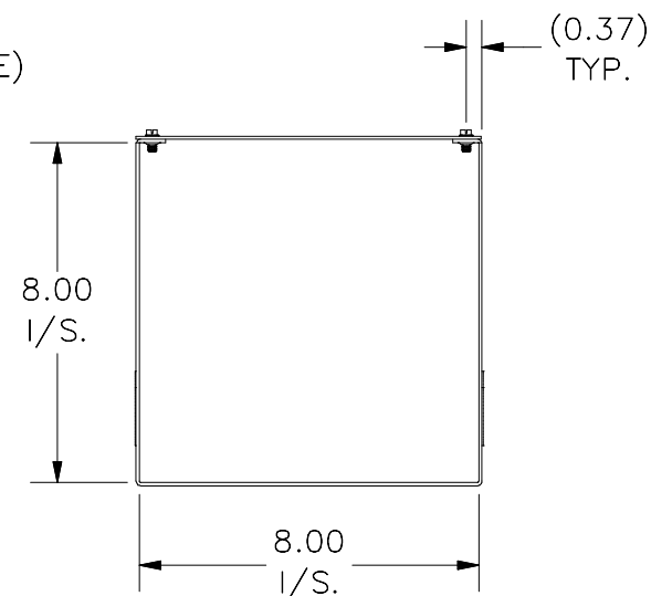
RIGHT VIEW
