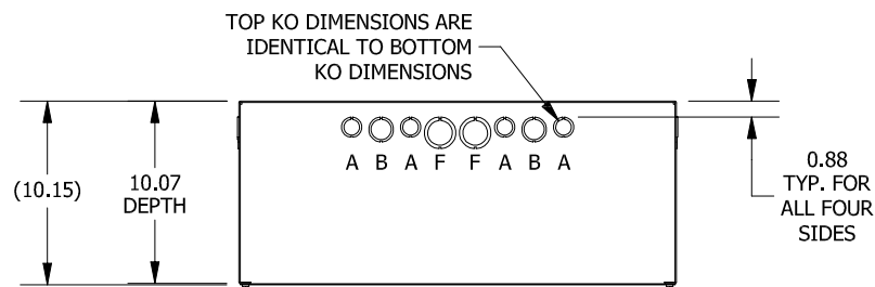
TOP VIEW
