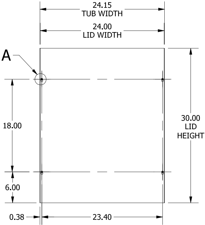
FRONT VIEW
