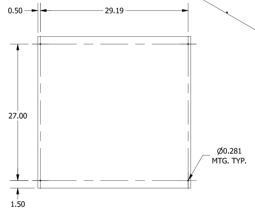
BACK VIEW
