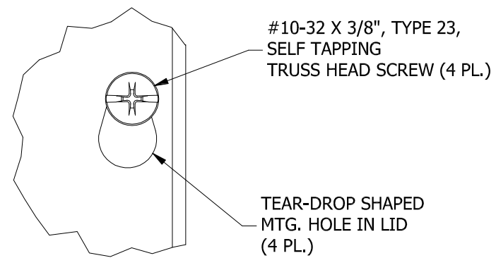
DETAIL C
