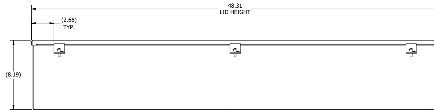
FRONT VIEW
