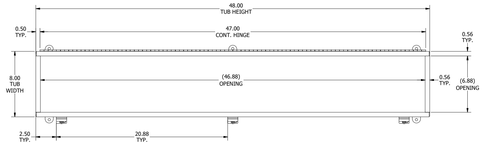
TOP VIEW (COVER REMOVED)
