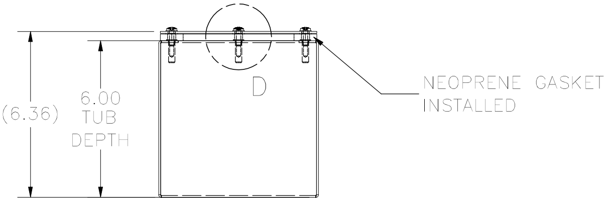
BOTTOM VIEW
