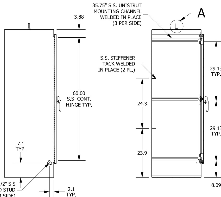
SECTION A-A (INSIDE RIGHT VIEW OF ENCL.)
