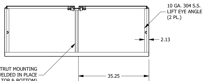
SECTION B-B (INSIDE TOP OF ENCL.)
