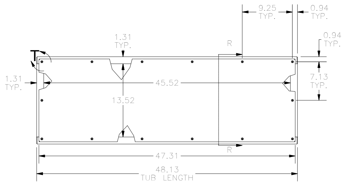
FRONT VIEW
