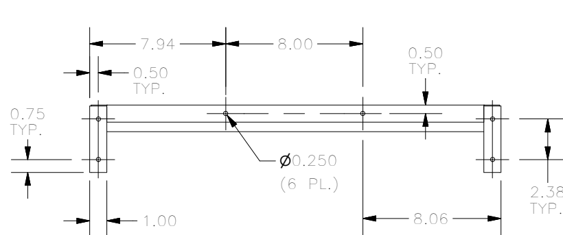
REAR VIEW
