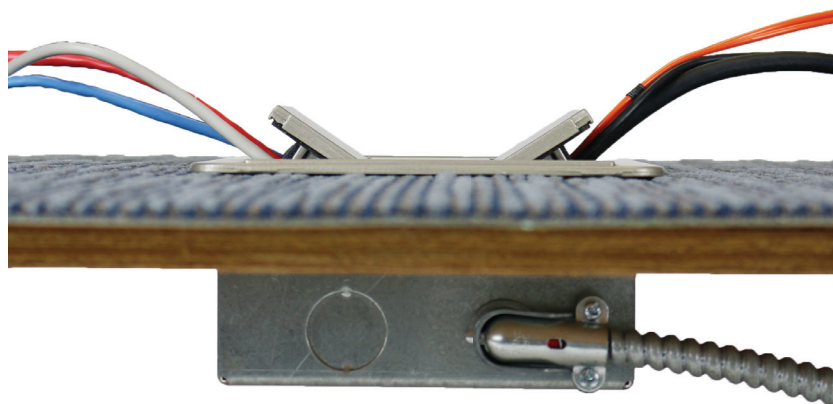
CAF3 installed in wood floor with Walkerflex® Wiring System.
