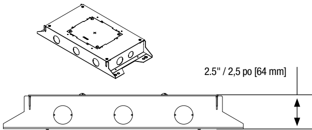
RFBA2R25 & RFBA2R25OG collar removed / sans collier / sin collarín
