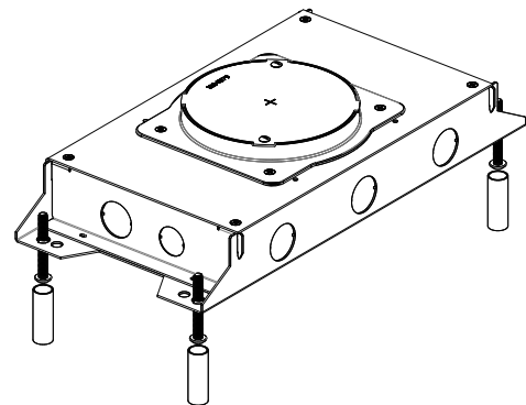
Leveling using \frac{1}{2} inch EMT and inverted leveling screws
